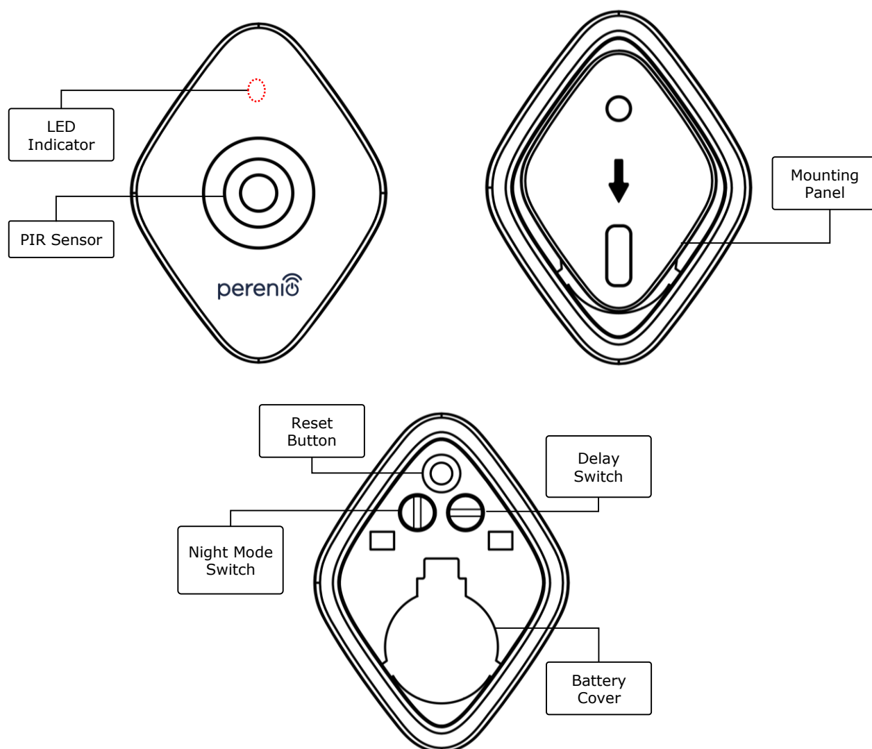
Figure 13 – PECMS01 Motion Sensor Exterior
