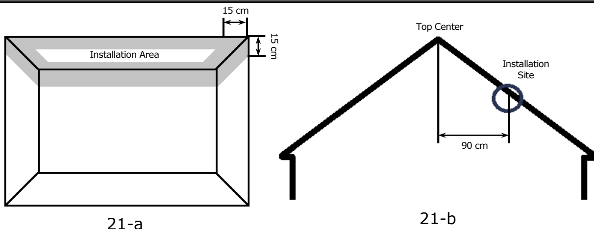
Figure 21 — Installation of the Smoke Sensor on a flat and sloping ceiling
