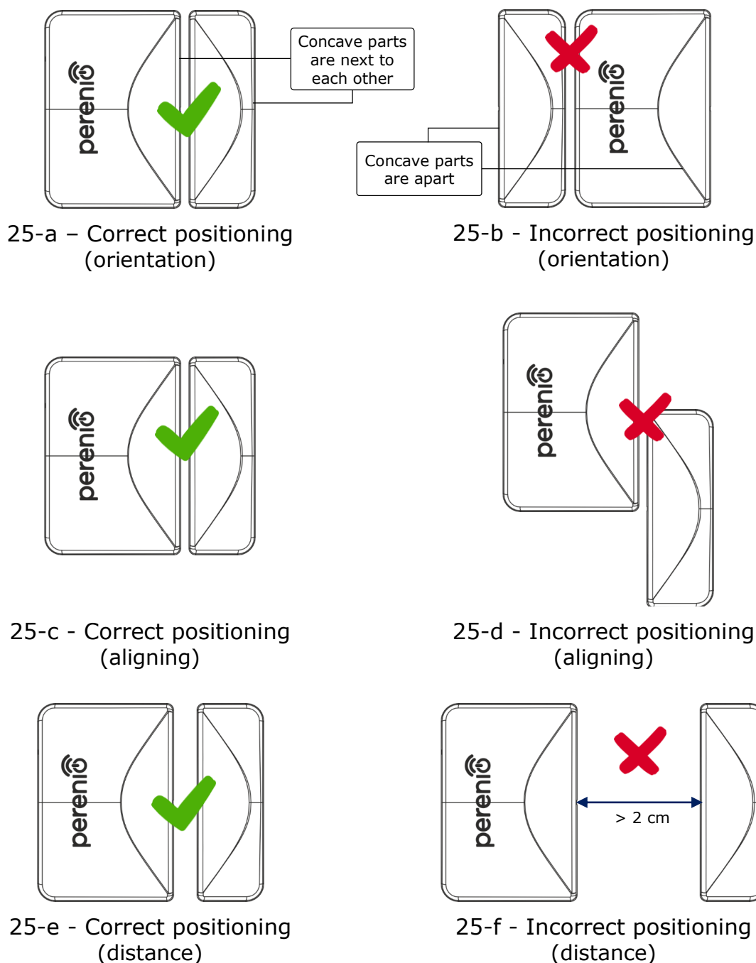
Figure 25 – Installation rules for the Sensor and the Magnet
