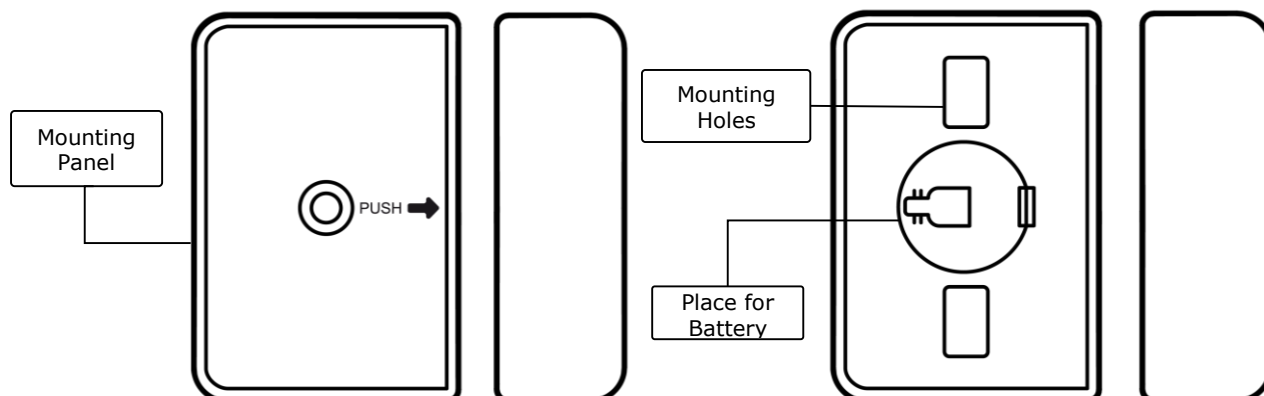
Figure 11 – PECWS01 Door & Window Sensor Components
