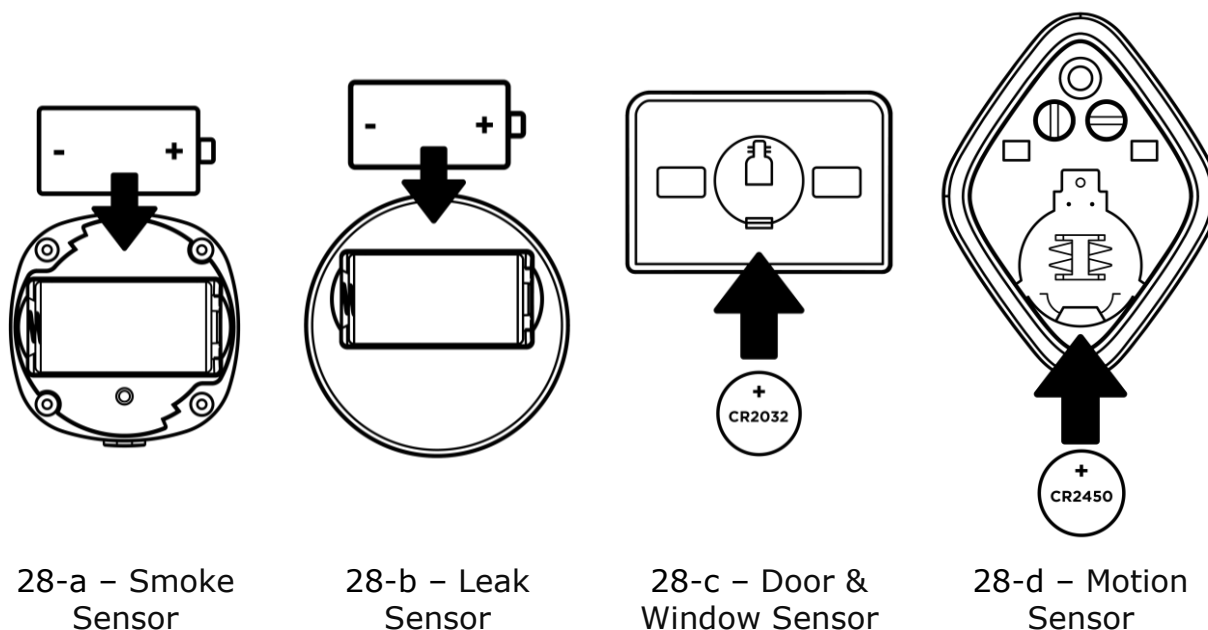
Figure 28 – Positioning of the battery in Sensors
