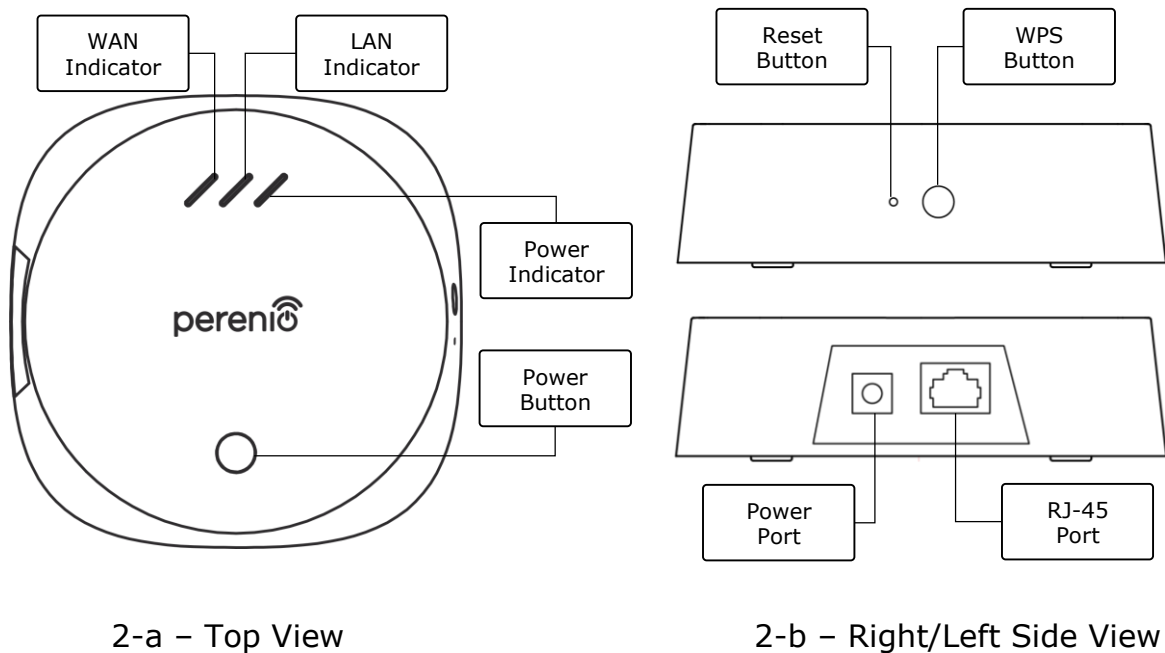
Figure 2 - The PEACG01 Control Gateway Buttons, Ports and Indicators
