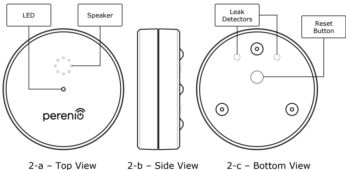
Figure 8 – PECLS01 Leak Sensor Buttons and Indicators
