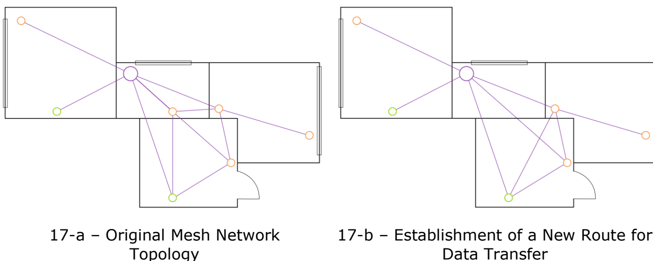
Figure 17 – Self-Recovery of the ZigBee Network
