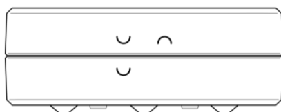
24-a – Initial position of the upper and lower parts of the Sensor body relative to each other (The Sensor is NOT CLOSED)
