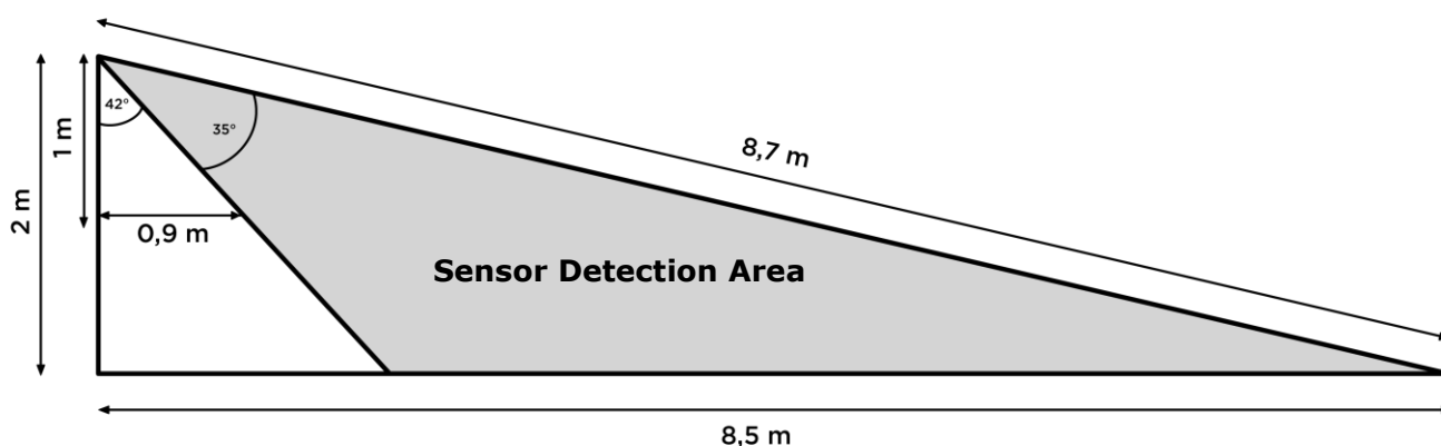
15-c – Details on the vertical detection angle
