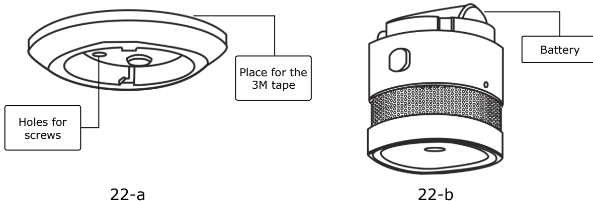
Figure 22 – Fastening of the Smoke Sensor on screws or the 3M tape
